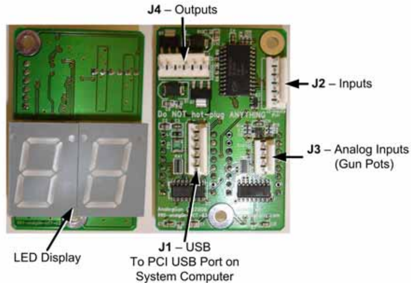
Figure 23. Gun PCB
