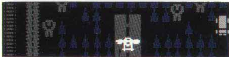
RUNWAY & PLANE
