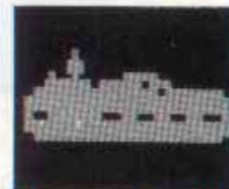
AIRCRAFT CARRIER
