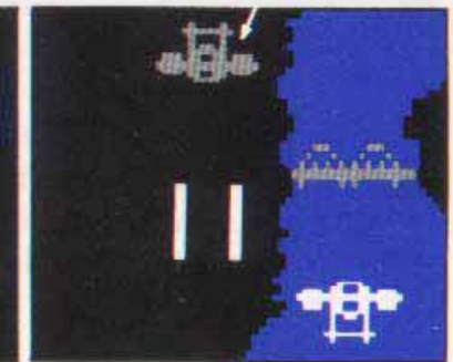
ENEMY PLANE
