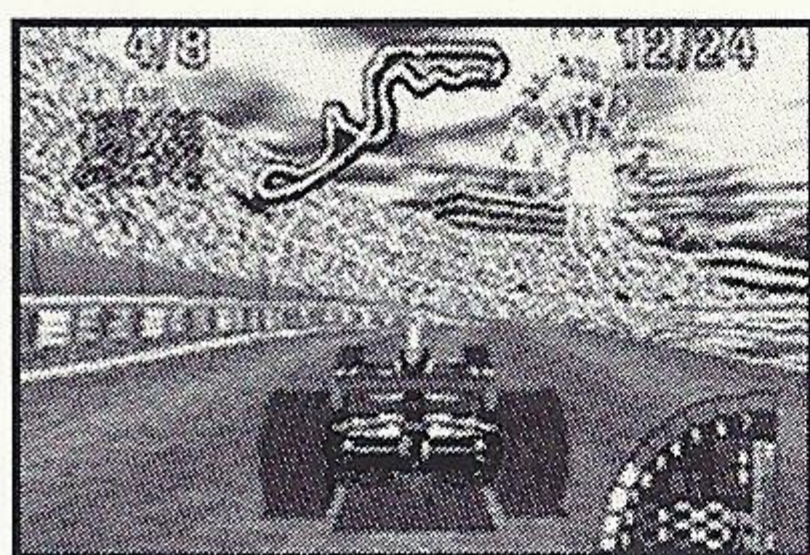
Suzuka
