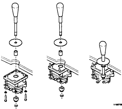
Figure 4: Joystick Installation
