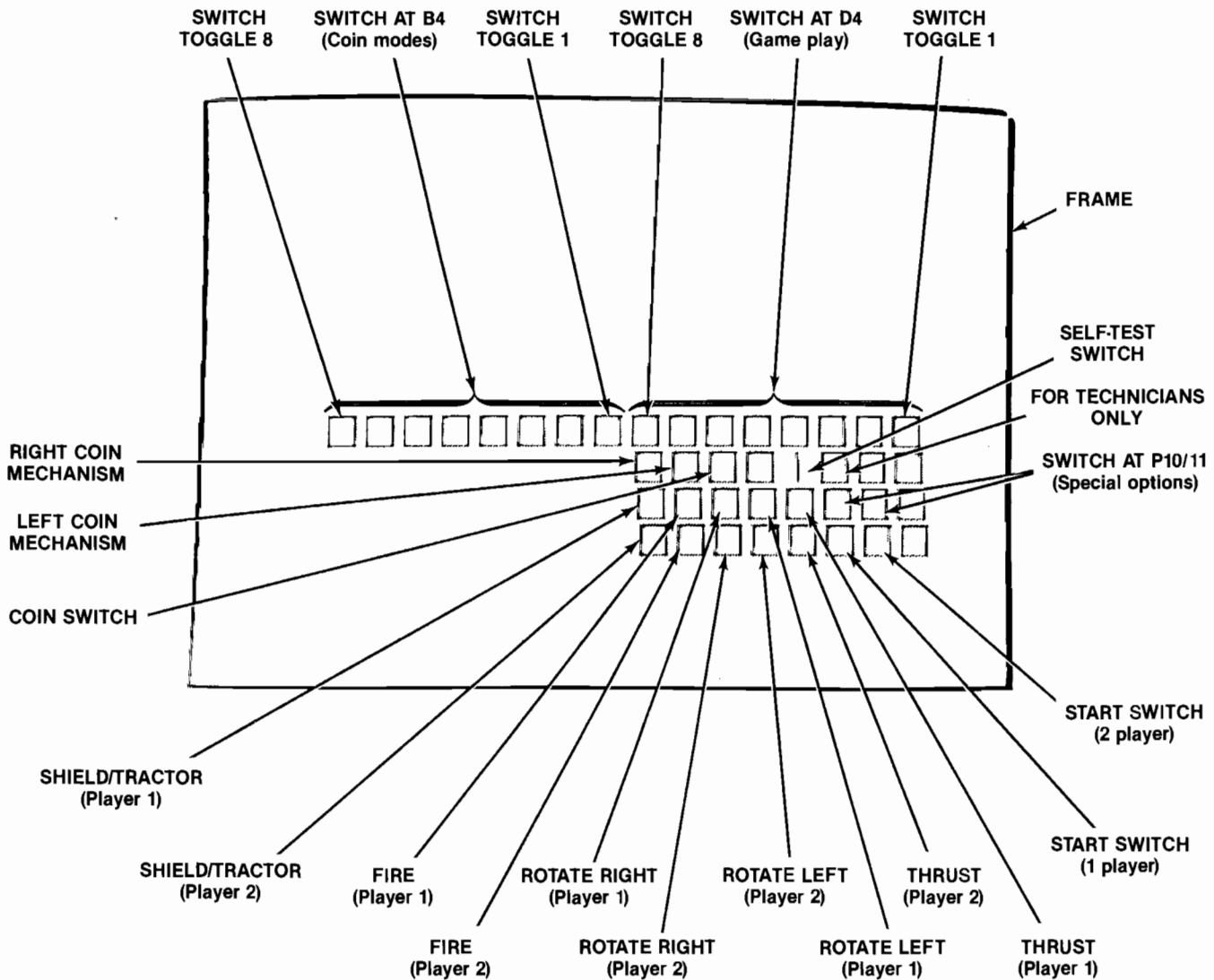
Figure 1-4 Self-Test Display
