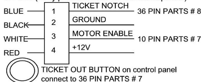
Ticket Dispenser Connection Diagram
