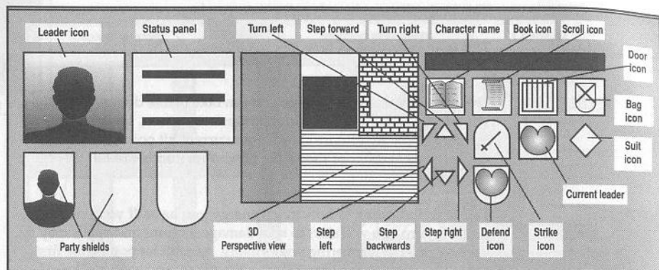
FIGURE TWO - THE MAIN SCREEN
